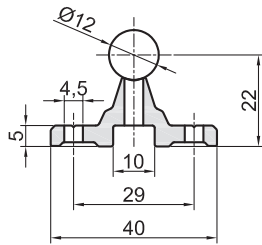
AD 12 (0,580 kg/m) ADWM 12 (1,570 kg/m)
