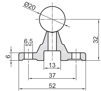
AD 20 (1,250 kg/m) ADWM 20 (3,710 kg/m)
