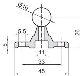
AD 16 (0,920 kg/m) ADWM 16 (2,530 kg/m)
